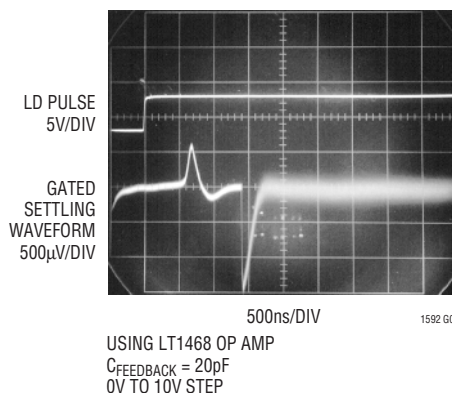
Full-Scale Settling Waveform
