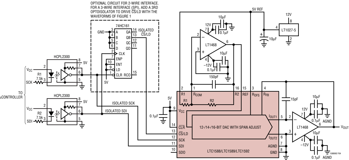
Figure 4. Optically Isolated 16-Bit SoftSpan System
