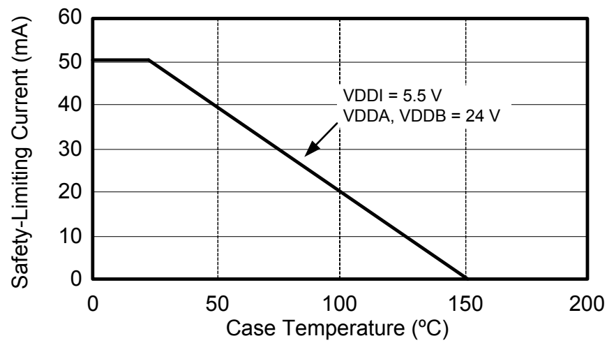
Figure 6. WB SOIC-16, NB SOIC-16, 14 LD LGA Thermal Derating Curve, Dependence of Safety Limiting Values with Case Temperature per DIN EN 60747-5-2
