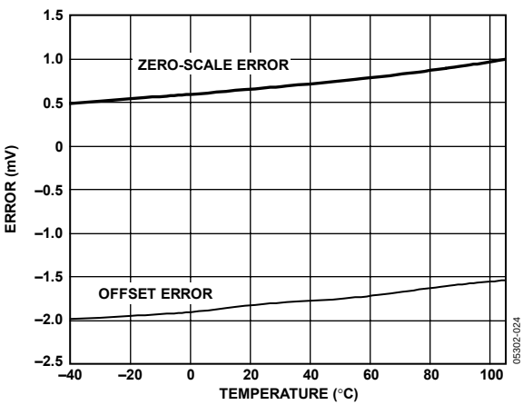
Figure 12. Zero-Scale and Offset Error vs. Temperature
