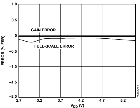
Figure 13. Gain Error and Full-Scale Error vs. Supply
