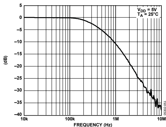
Figure 31. Multiplying Bandwidth
