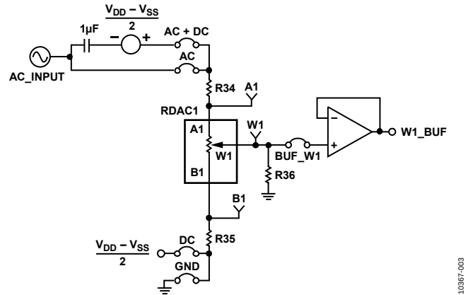
Figure 3. AC Signal Attenuator
