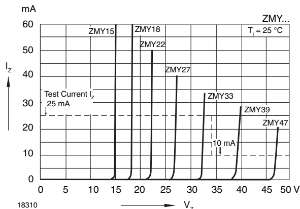
Fig. 7 - Breakdown Characteristics
