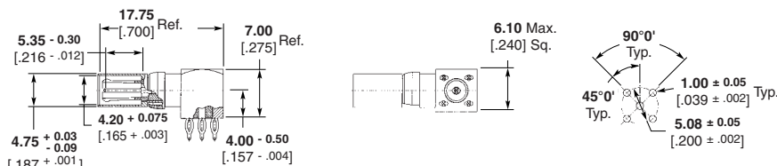
Recommended PC Board Layout
