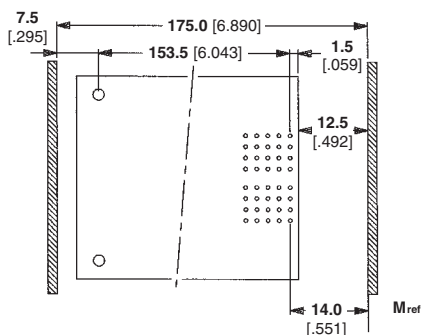
Coordination Dimensions
