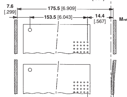
Subrack tolerances
