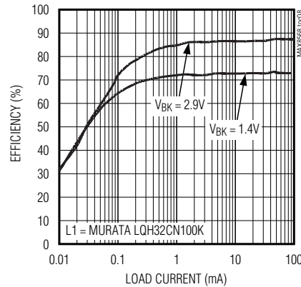
2.5V STEP-UP EFFICIENCY vs. LOAD CURRENT
