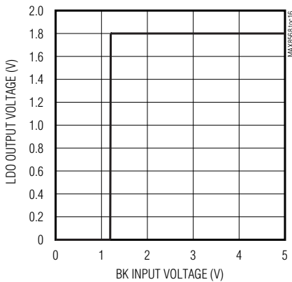
LDO OUTPUT VOLTAGE vs. BK INPUT VOLTAGE
