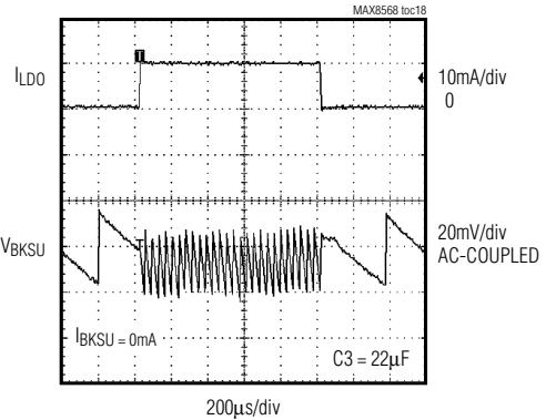
BKSU RESPONSE TO LDO LOAD TRANSIENT
