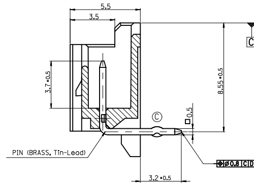
SECTION K-K'
