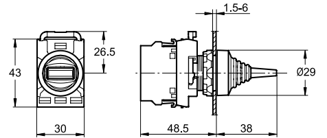
Toggle Switch
