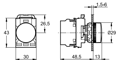
Pilot Light
