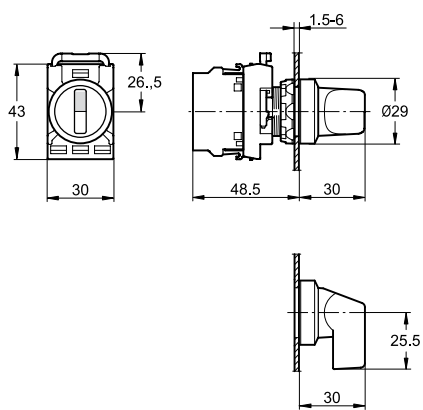
Selector Switch
