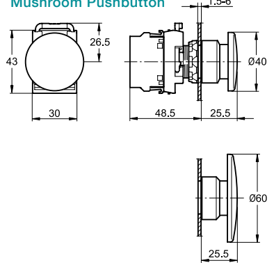
Mushroom Pushbutton
