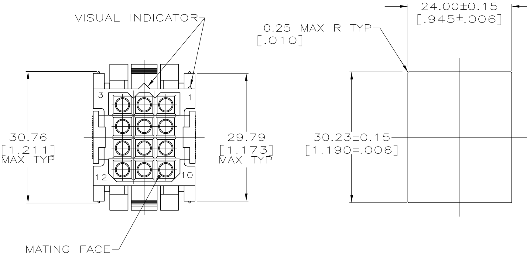
PANEL CUTOUT
