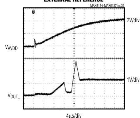
POWER-UP GLITCH, MIDSCALE, EXTERNAL REFERENCE
