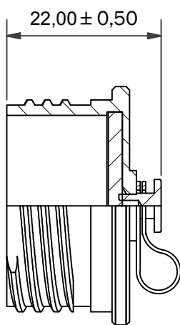
100P237-17-1-C-EO EYELET ONLY VERSION (EYELET SIZE OPTIONS NOT AVAILABLE)
