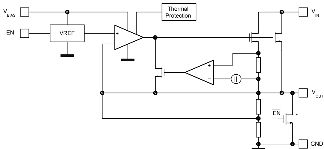
Figure 2. Block diagram
