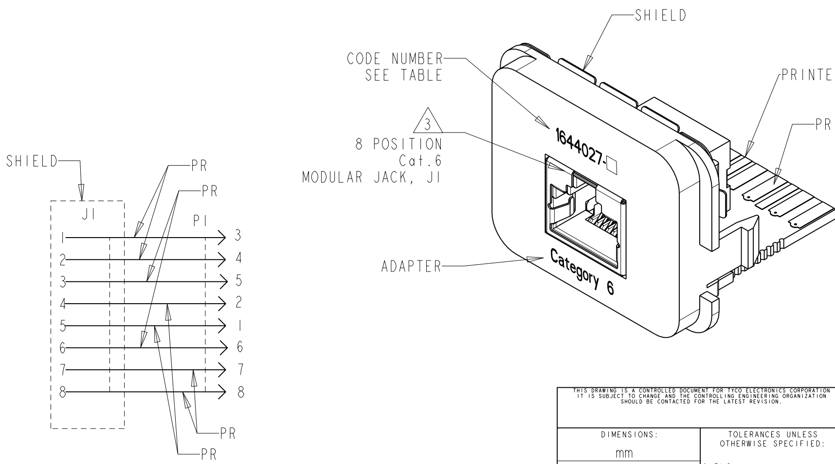
ELECTRICAL SCHEMATIC
