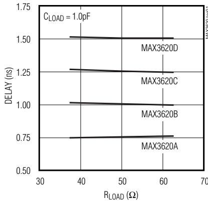
DELAY vs. R_{LOAD} (LOW LOAD RESISTANCE)
