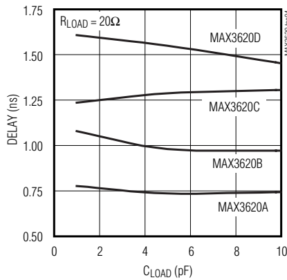
DELAY vs. C_{LOAD} (HIGH LOAD RESISTANCE)
