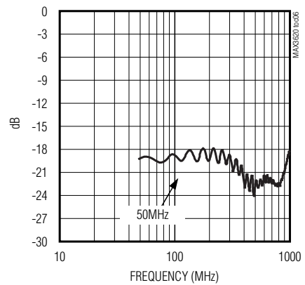
MAX3620B S11
