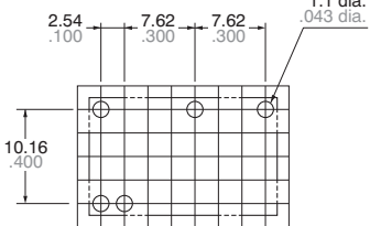
2 coil latching
