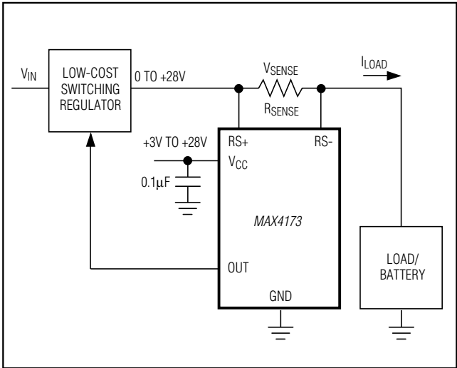
Figure 3. Current Source
