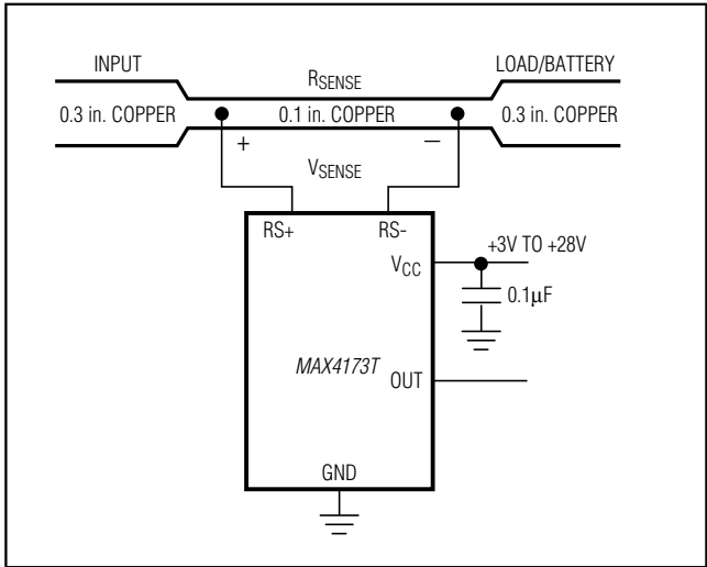
Figure 2. MAX4173 Connections Showing Use of PC Board
