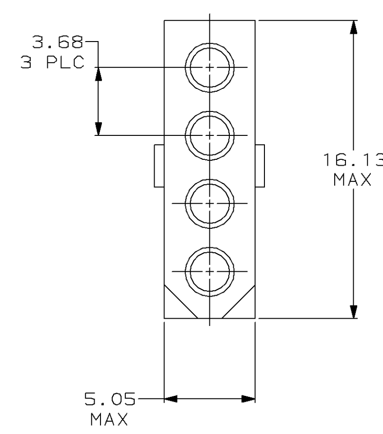
MATING CONNECTOR INTERFACE
