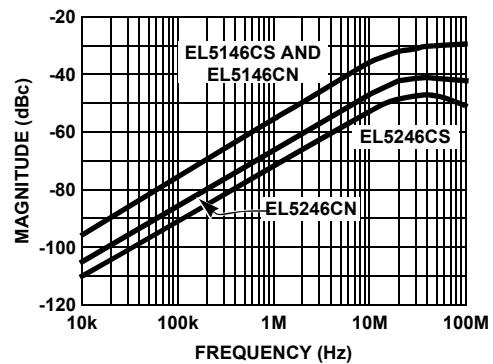
FIGURE 44. OFF ISOLATION - EL5146 AND EL5246
