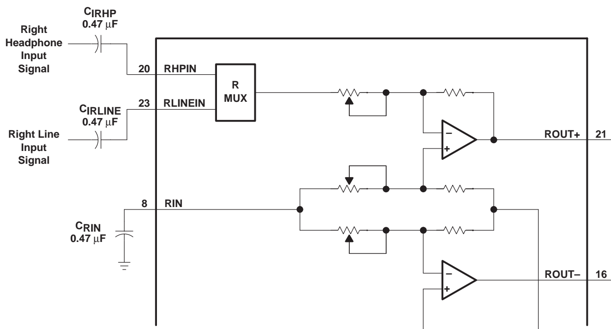
Figure 48. TPA0112 Example Input MUX Circuit
