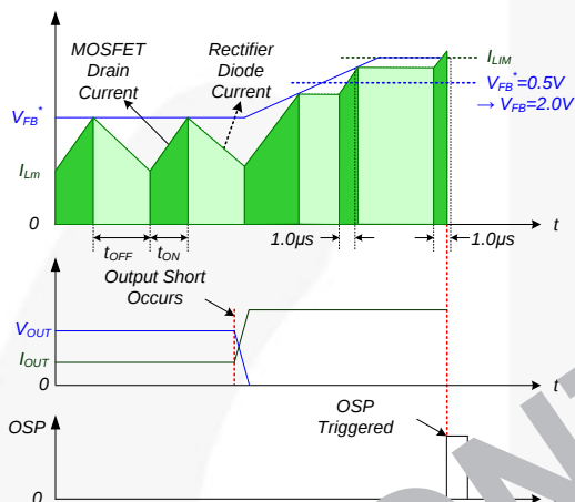
Figure 24. Output-Short Protection
