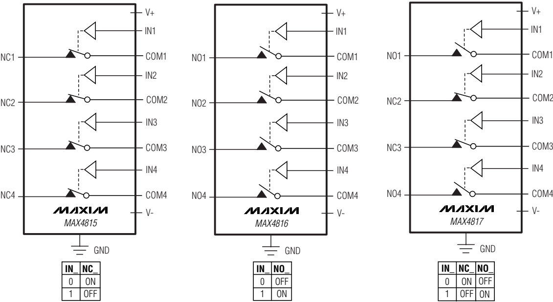
Functional Diagram
