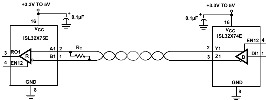
FIGURE 4. NETWORK USING PAIRED ENABLES
