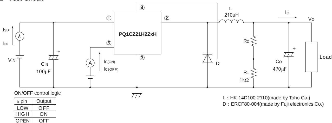
Fig.1 Test Circuit
