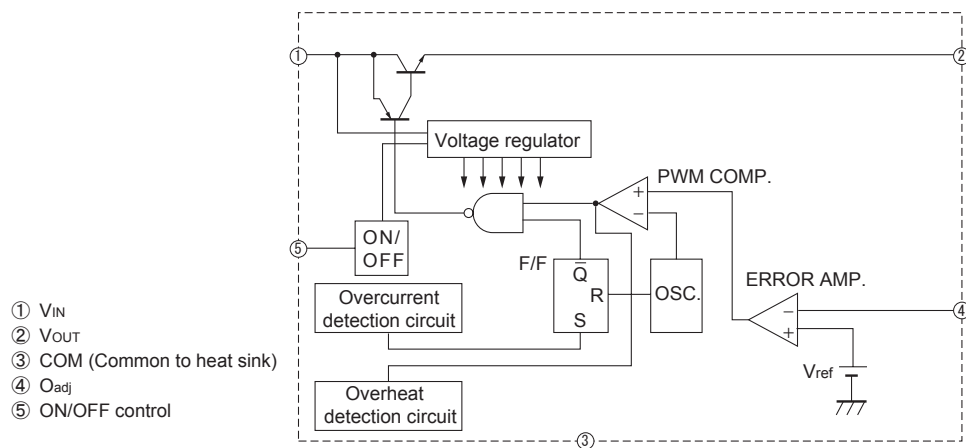
Fig.14 Block Diagram
