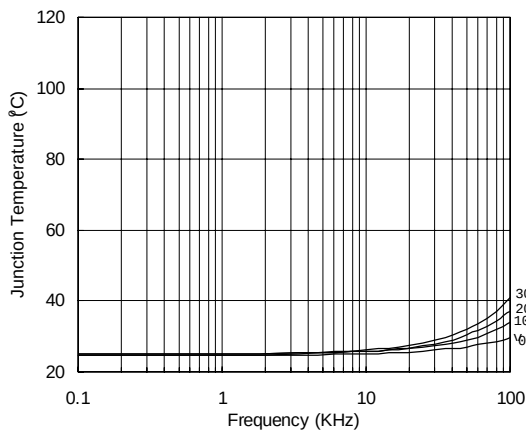
Figure 49. IR2136/IR21362(3)(5)(6)(7)(8) (S) vs. Frequency (IRG4BC20W), Rgate=33Ω, Vcc=15V
