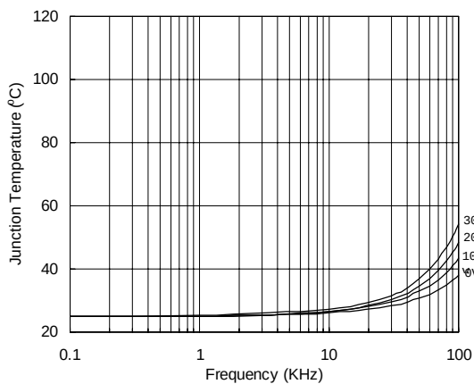
Figure 51. IR2136/IR21362(3)(5)(6)(7)(8) (S) vs. Frequency (IRG4BC40W), Rgate=10Ω, Vcc=15V
