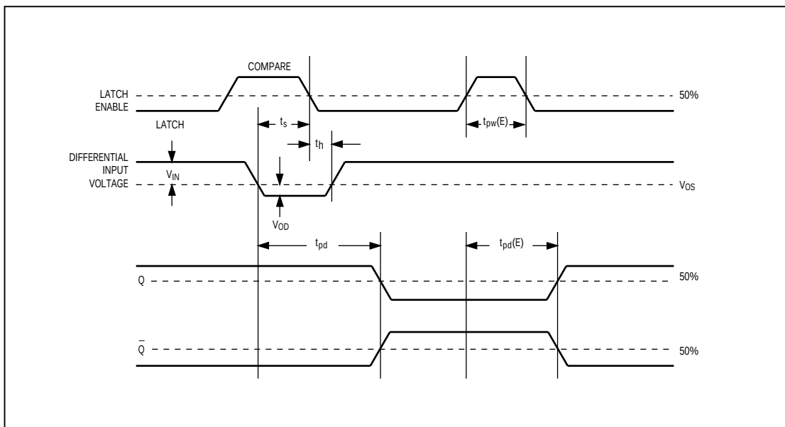
Figure 3. Timing Diagram
