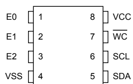
Figure 2. 8-pin package connections
