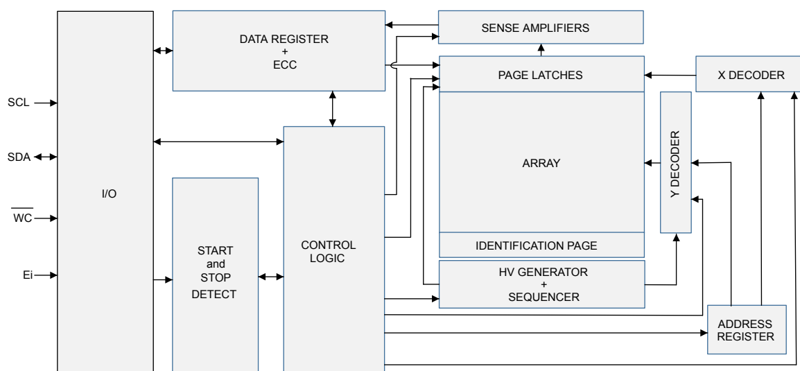
Figure 1. Logic diagram
