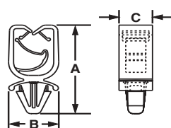
Vertical HCMP06B12
