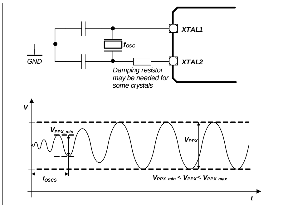
Figure 16 Oscillator in Crystal Mode
