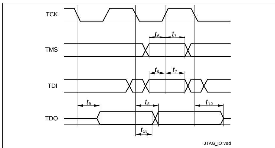
Figure 24 JTAG Timing
