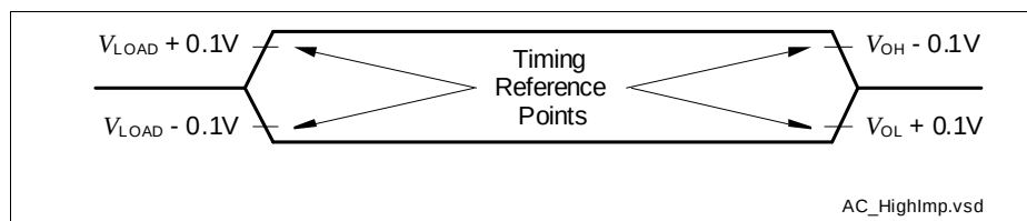
Figure 20 Testing Waveform, Output High Impedance
