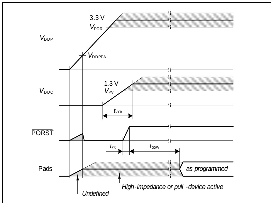
Figure 22 Power-Up Behavior
