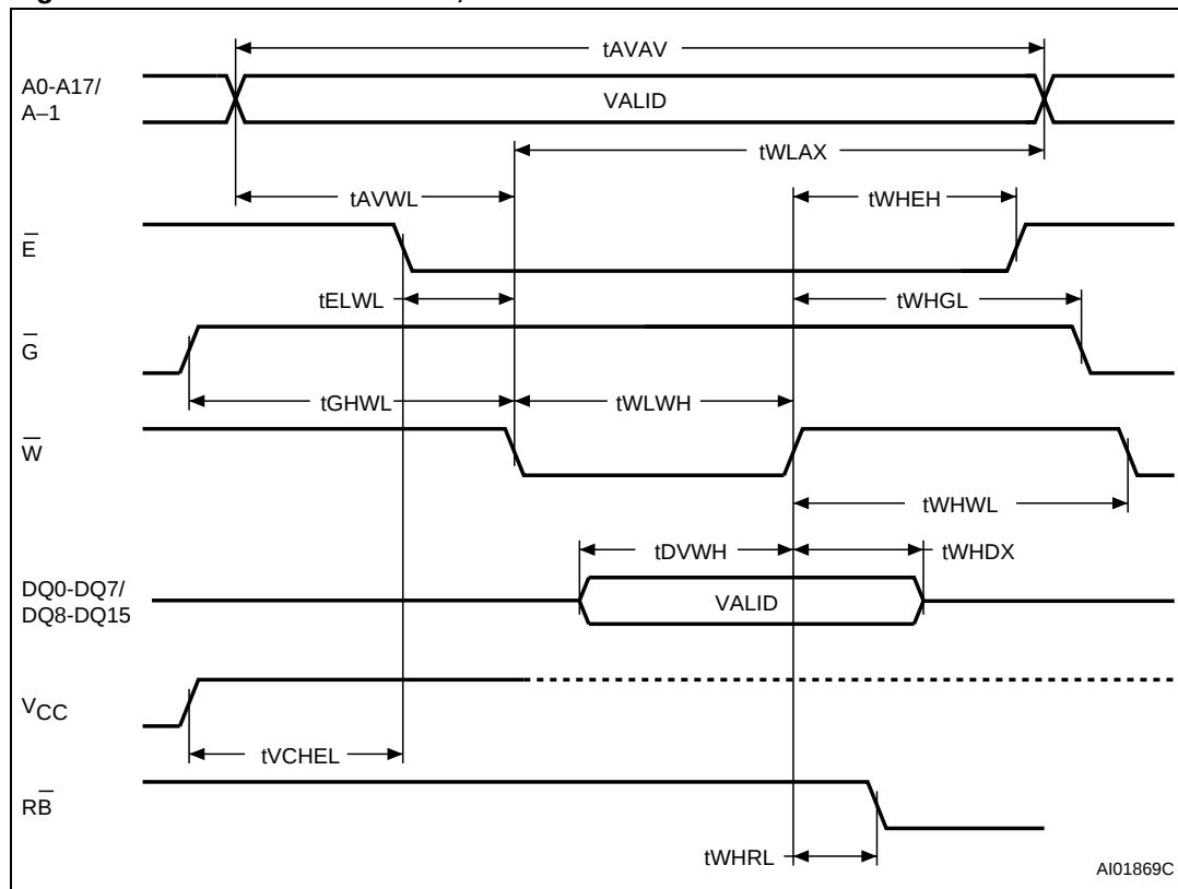
Figure 9. Write AC waveforms, Write Enable controlled
