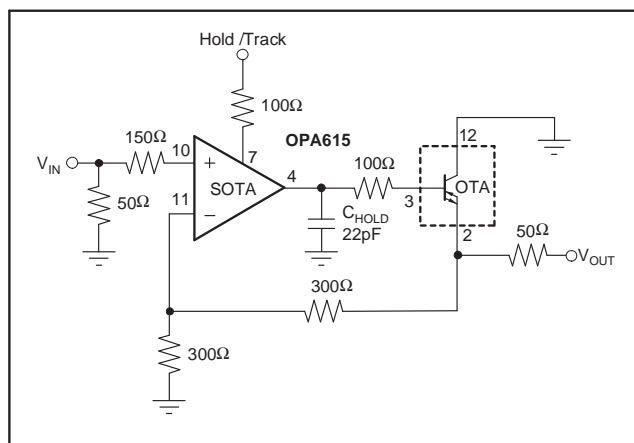
Figure 45. Sample-and-Hold Amplifier
