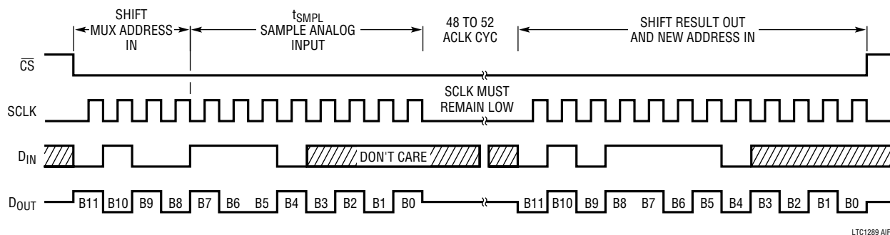
Figure 4. \overline{CS} Low During Conversion
