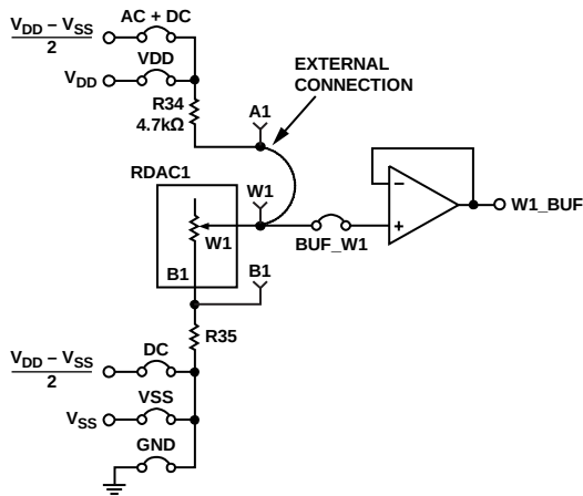
Figure 2. Pseudologarithmic DAC
