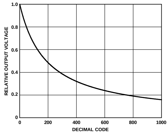
Figure 5. Pseudoantilogarithmic Gain
