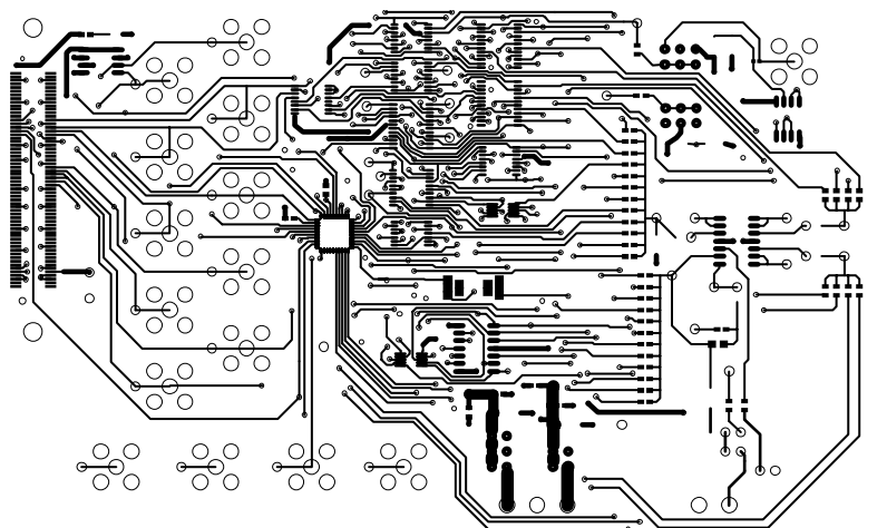
Figure 17. Component Placement Drawing
