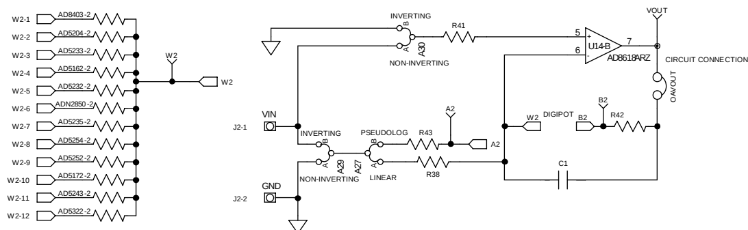
Figure 13. Schematic of Multiboard RDAC2 Circuits
