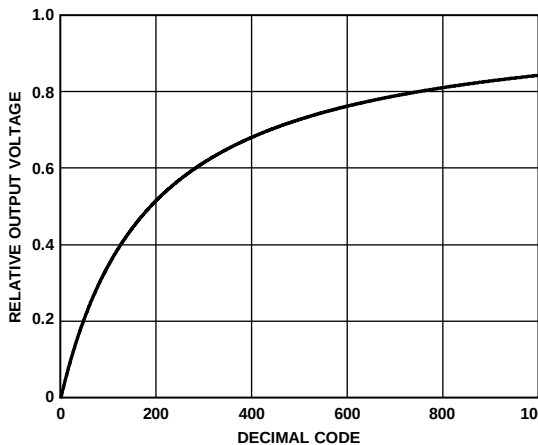
Figure 3. Pseudologarithmic Gain
