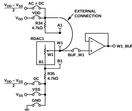
Figure 4. Pseudoantilogarithmic DAC.
