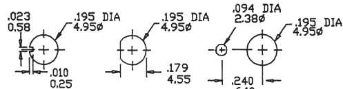
Without locking ring
