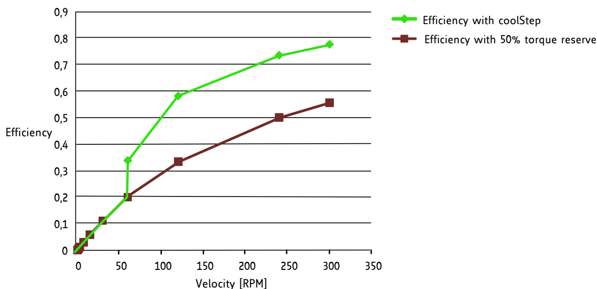
Figure 5.1 Energy efficiency example with coolStep
