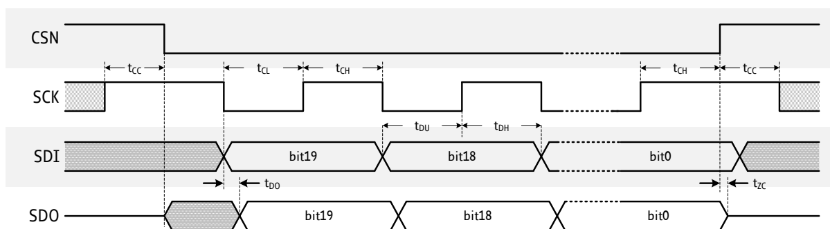
Figure 6.1 SPI Timing
