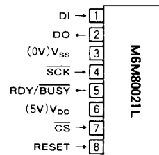
Outline 8P5K
