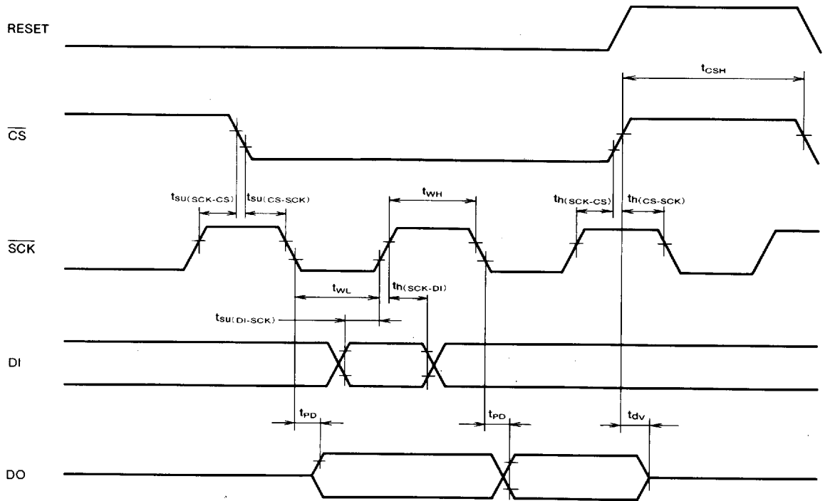
Fig. 1 Synchronizing timing
