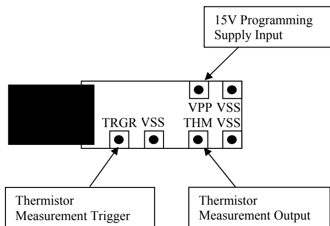
Figure 2: DS2703 EV Kit (PD122404 ) Connections
