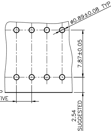
SECTION HH
