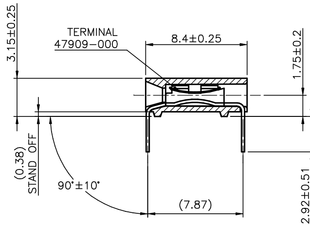
SECTION HH
