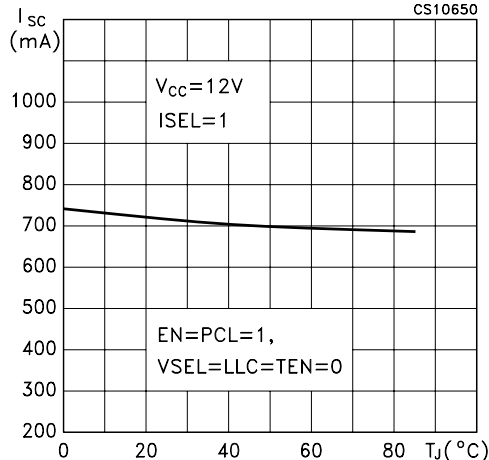
Figure 19: Output Current Limiting vs Temperature
