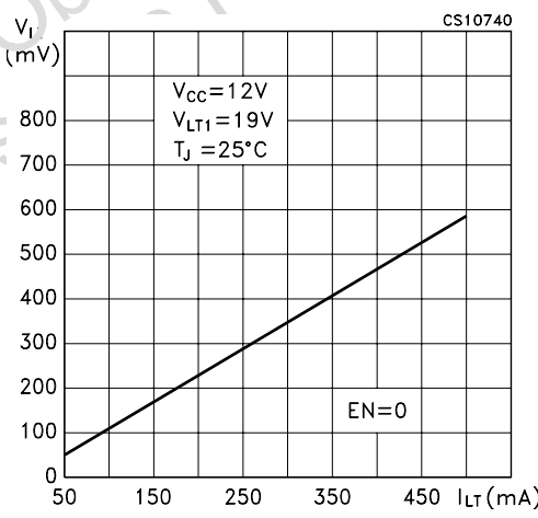
Figure 28: Loophthrough Switch Drop Voltage vs Loophthrough Current
