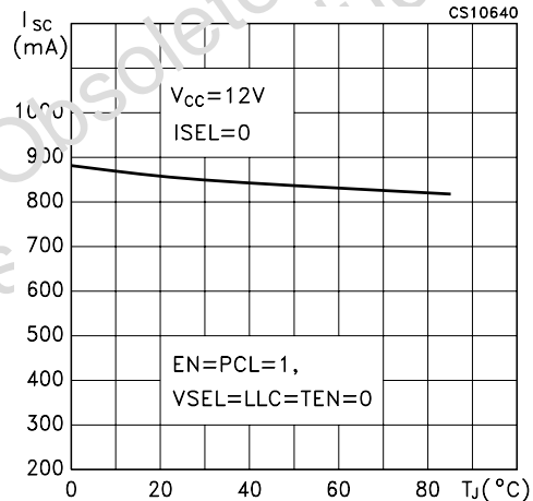
Figure 18: Output Current Limiting vs Temperature
