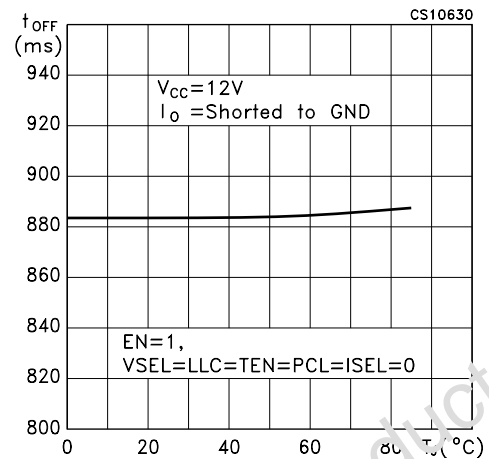
Figure 17: Dynamic Overload Protection OFF Time vs Temperature
