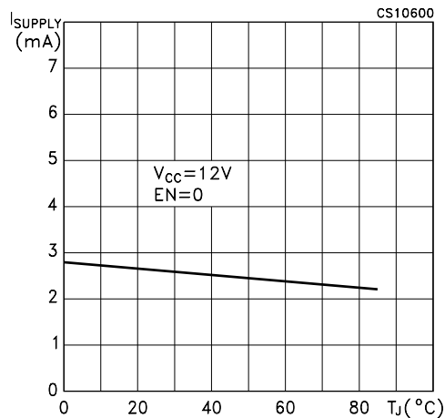
Figure 15: Supply Current vs Temperature
