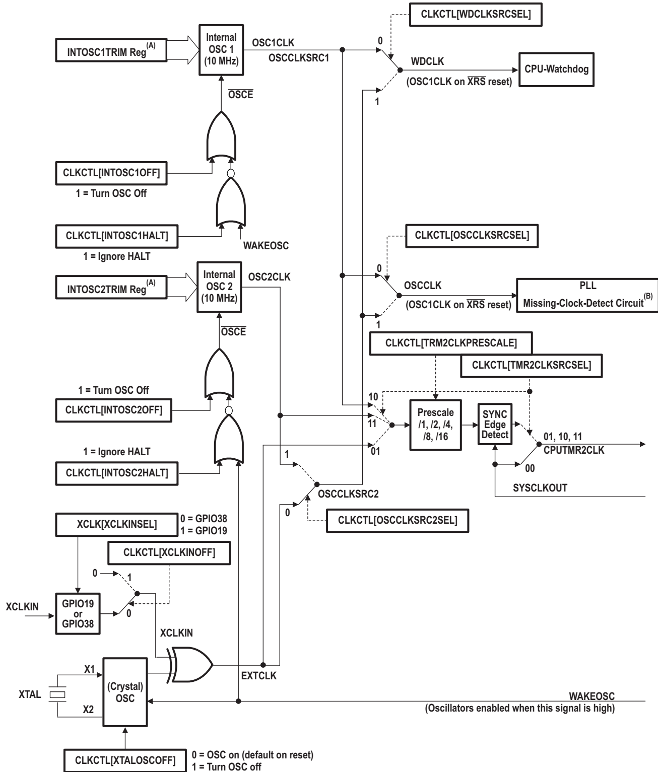
Figure 3-9. Clock Tree
