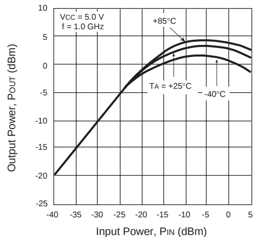
UPC2712TB OUTPUT POWER vs. INPUT POWER AND TEMPERATURE
