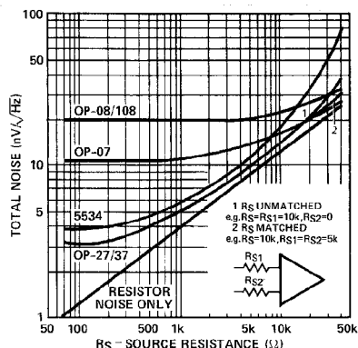
NOISE vs SOURCE RESISTANCE (INCLUDING RESISTOR NOISE) AT 1000Hz
