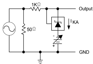
TEST CIRCUIT FOR REFERENCE IMPEDANCE
