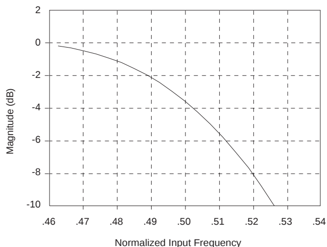
Figure 6. CS5330A/31A Digital Filter Transition Band
