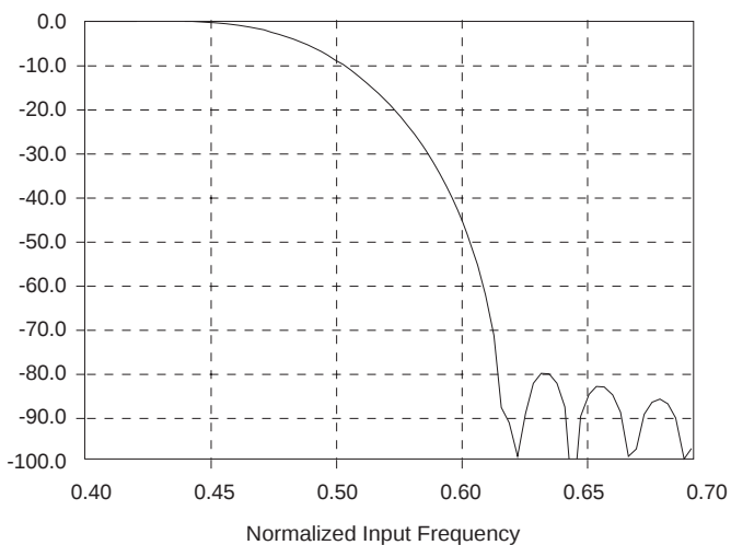
Figure 8. CS5330A/31A Digital Filter Transition Band
