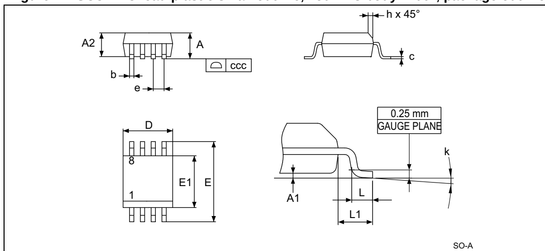
Figure 74. SO8N – 8-lead plastic small outline, 150 mils body width, package outline
