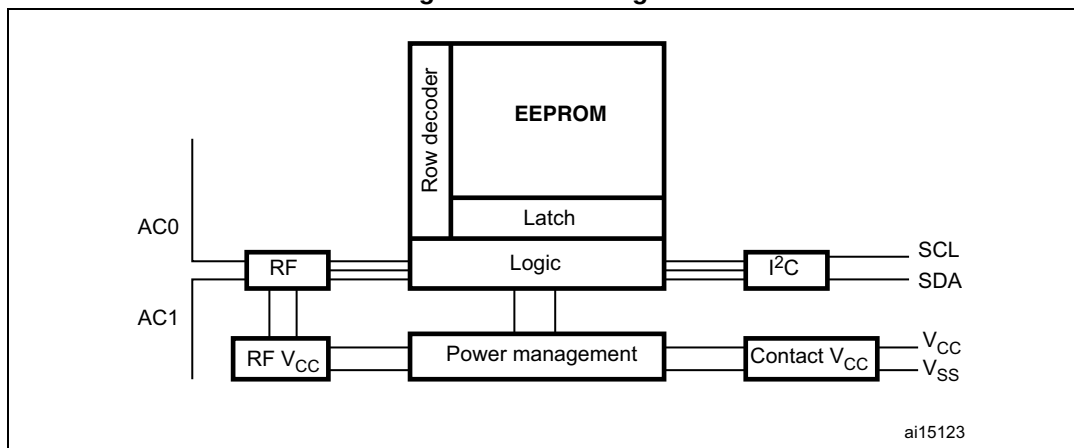
Figure 6. Block diagram
