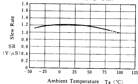
Slew Rate vs. Temperature
