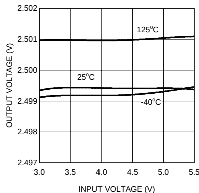
Figure 50. Line Regulation
