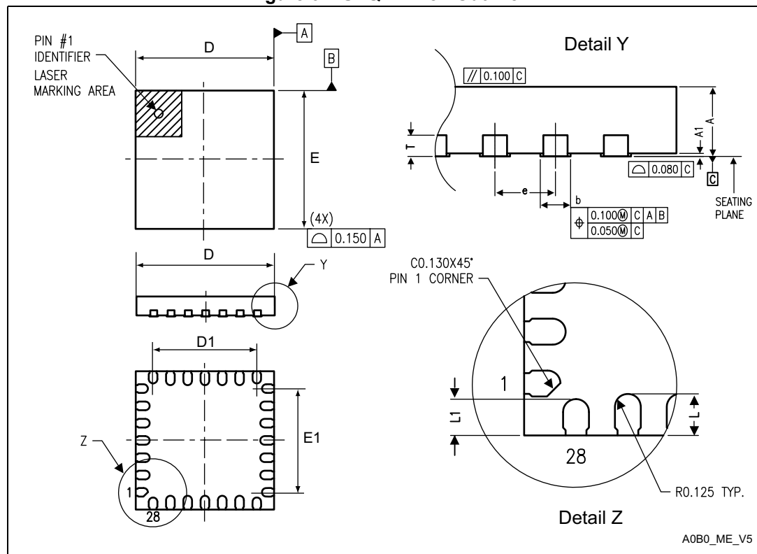
Figure 37. UFQFPN28 - Outline
