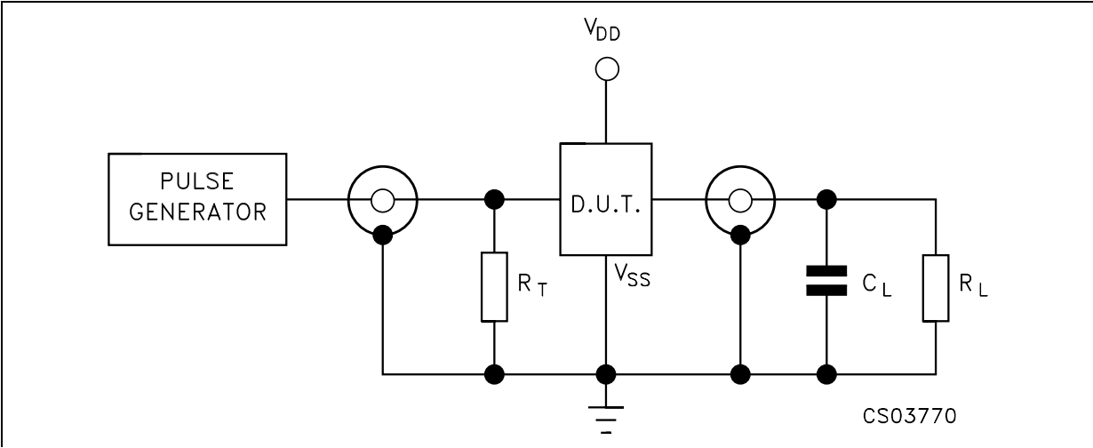
TEST CIRCUIT
