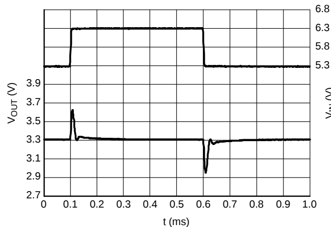
Figure 31. Line Transients, 3.3 V Version, t_R = t_F = 5 \mu\text{s} , I_{\text{OUT}} = 30 \text{ mA}
