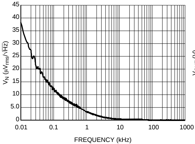
Figure 29. Output Voltage Noise, 12.0 V Version, V_{\text{IN}} = 14.0 \text{ V} , I_{\text{OUT}} = 30 \text{ mA}
