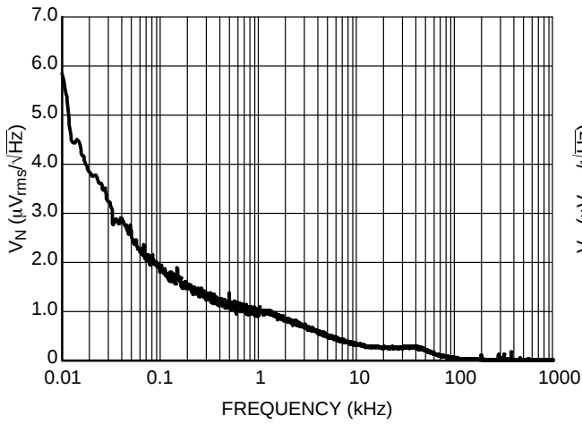
Figure 27. Output Voltage Noise, 3.3 V Version, V_{\text{IN}} = 5.3 \text{ V} , I_{\text{OUT}} = 30 \text{ mA}
