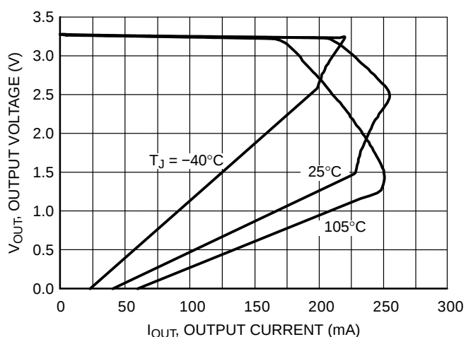
Figure 4. Output Voltage vs. Output Current 3.3 V Version V_{IN} = 5.3\text{ V}
