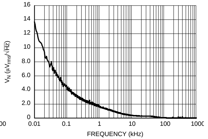
Figure 28. Output Voltage Noise, 5.0 V Version, V_{\text{IN}} = 7.0 \text{ V} , I_{\text{OUT}} = 30 \text{ mA}
